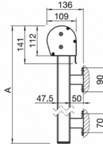
Wall fixing
