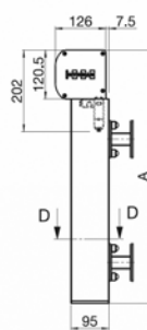
Wall fixing with brackets
