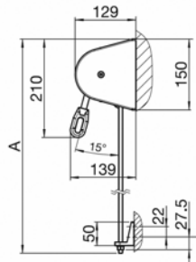
Wall fixing
