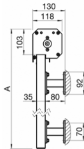
Wall fixing
