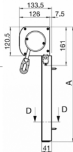
Wall fixing with clip system
